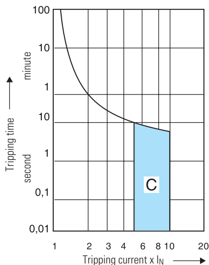
Tripping characteristic C curve
