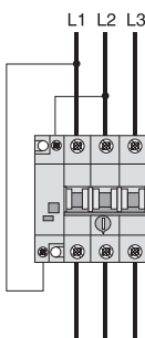
Wiring Example Z-USA/400+FAZ
