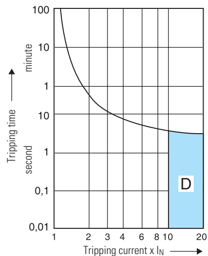
Tripping characteristic D curve
